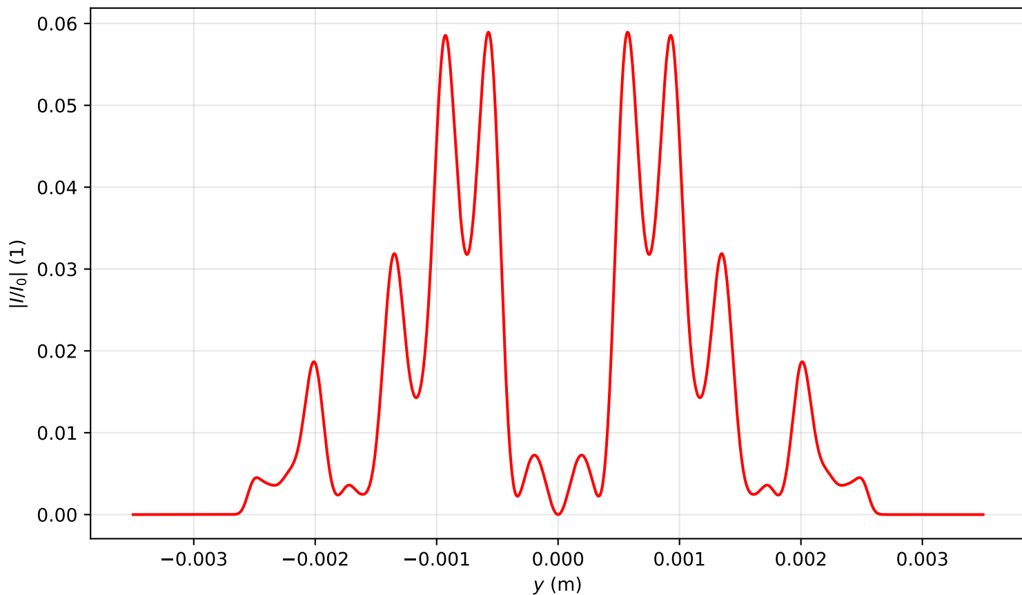
Intensity profile I(x=0, y, z=3.184)/I_0 , \text{Pin}=8.0\text{Pcr} , artificial time
